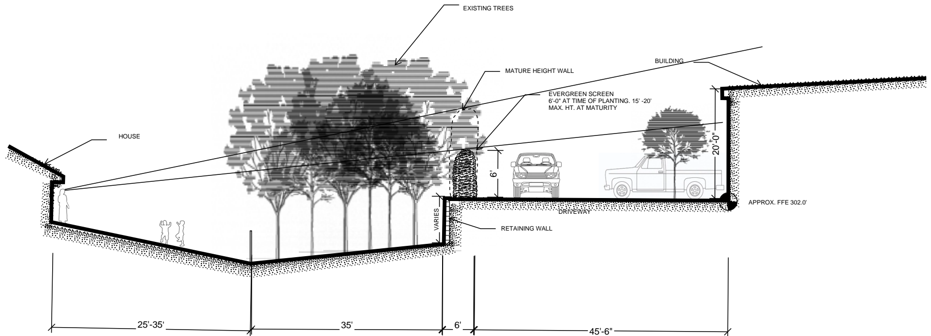
SECTION A
